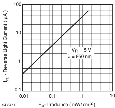
Fig. 4 Reverse Light Current vs. Irradiance
